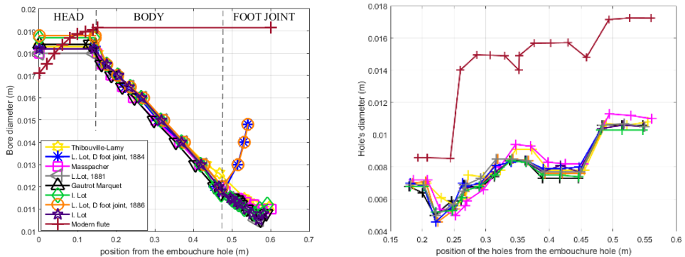
Figure 1: left - bore diameters of the flutes, right – hole’s diameter and position from the embouchure hole.
